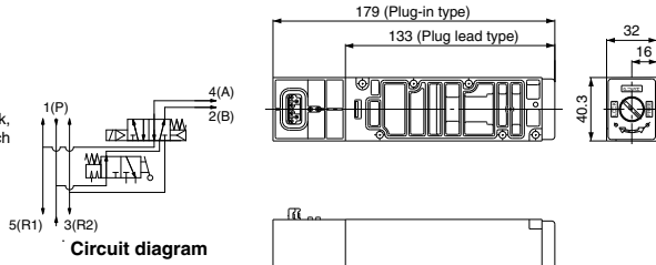
Circuit diagram
