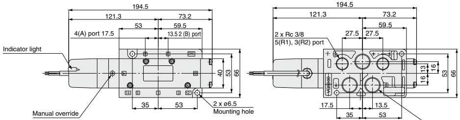
Bottom ported drawing 3 x Rc 1/2 1(P), 4 (A), 2 (B) port
