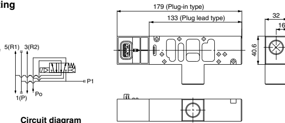
Circuit diagram
