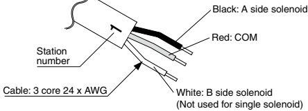
Single solenoid
