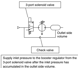
Recommended air circuit
