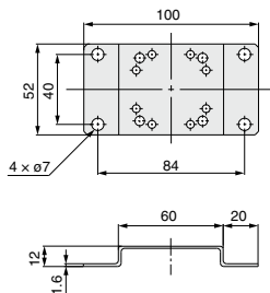
Flat bracket
