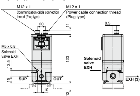
Straight type (4 cores) Cable connector 3 m
