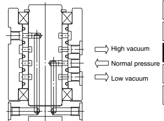
Using normal pressure port
