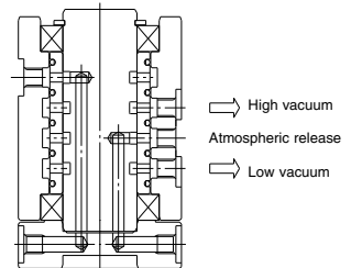
Using atmospheric release port
