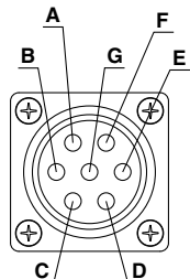
DC connector (HED007-C2□, HED009-C2□)
